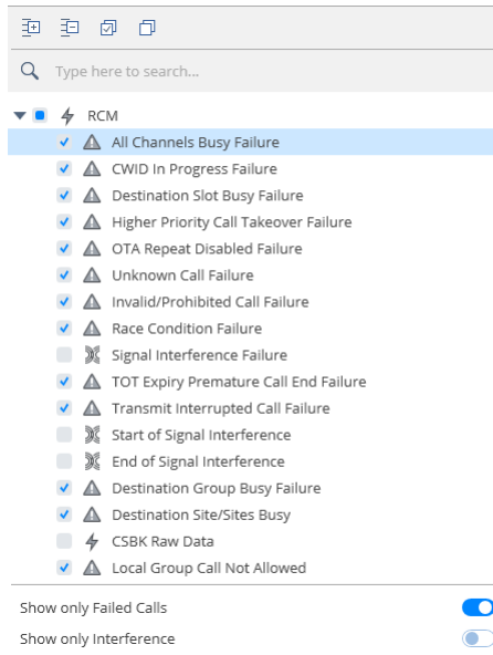
Figure 58: RCM section
