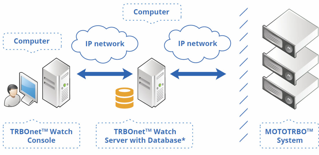
Figure 1: TRBOnet Watch architecture
