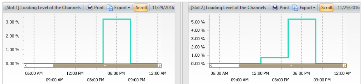
Figure 91: The loading level in the time slots of a MOTOTRBO IPSC system
