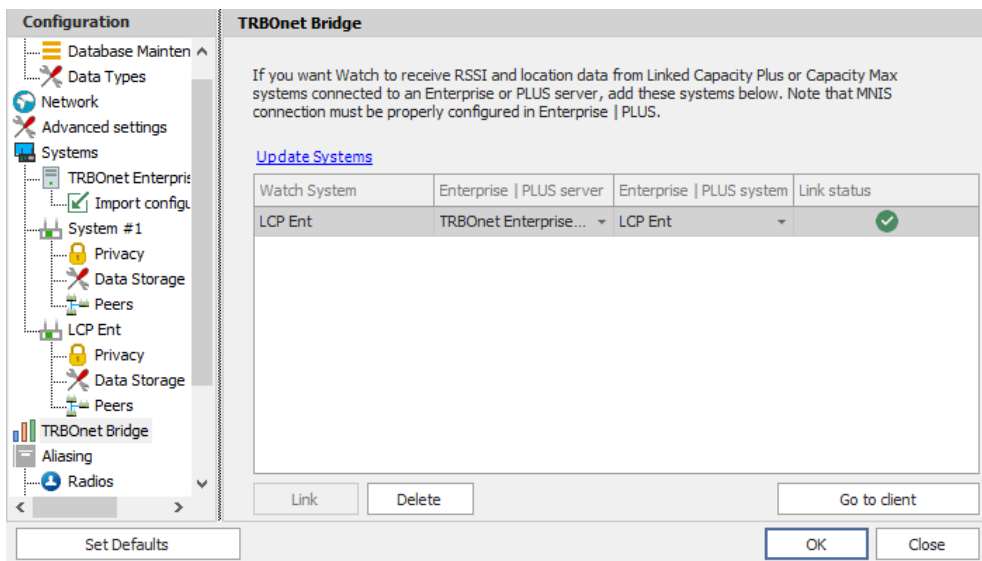
Figure 26: TRBOnet Bridge
