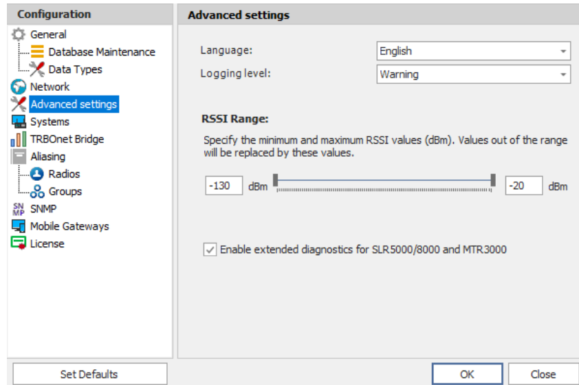
Figure 9: Advanced settings
