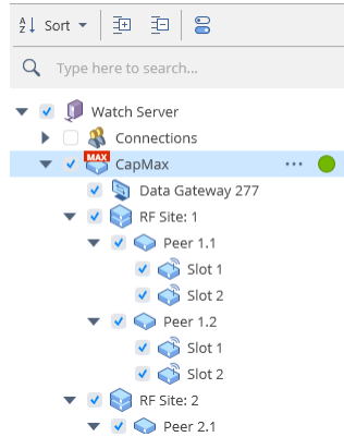
Figure 53: Left pane
