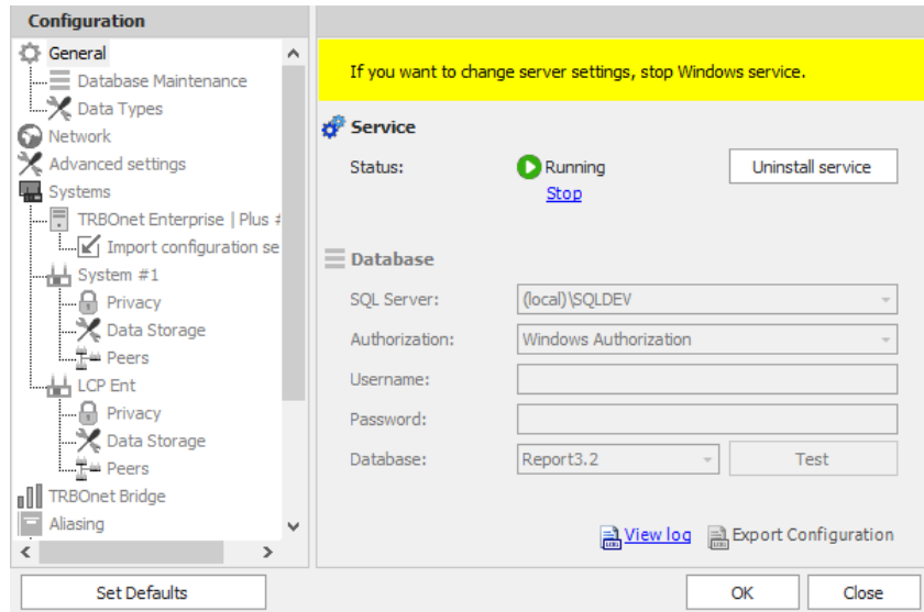
Figure 32: Service started
