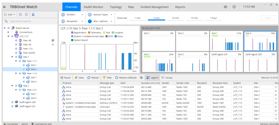
Figure 52: Channels tab
