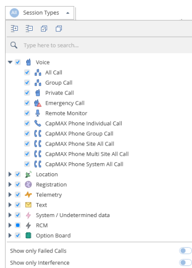
Figure 57: Session types
